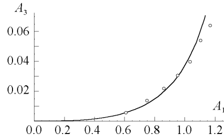
Figure 7. The third harmonic amplitude for n = 8 mode versus the amplitude of the principal harmonic given by the approximate theory (see text) and by the simulation experiment.
