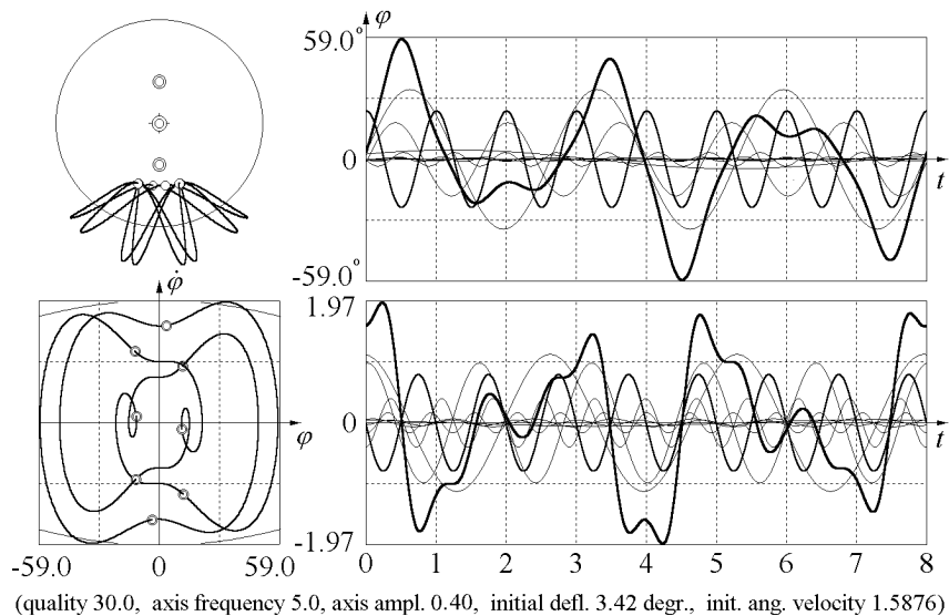
Figure 14. The spatial path, phase orbit, and graphs of stationary oscillations that can be treated as a subharmonic resonance of a fractional order 8/3 . The third harmonic (frequency 3\omega/8 ) dominates in the spectrum.
